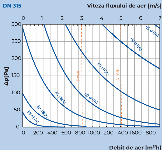
DN 315
