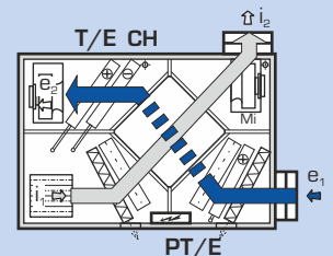
Ventilation without heat recovery (via bypass)
