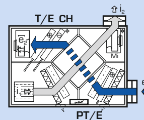
Ventilation without heat recovery (via bypass)
