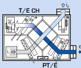
Ventilation with heat recovery with heating, cooling and preheating
