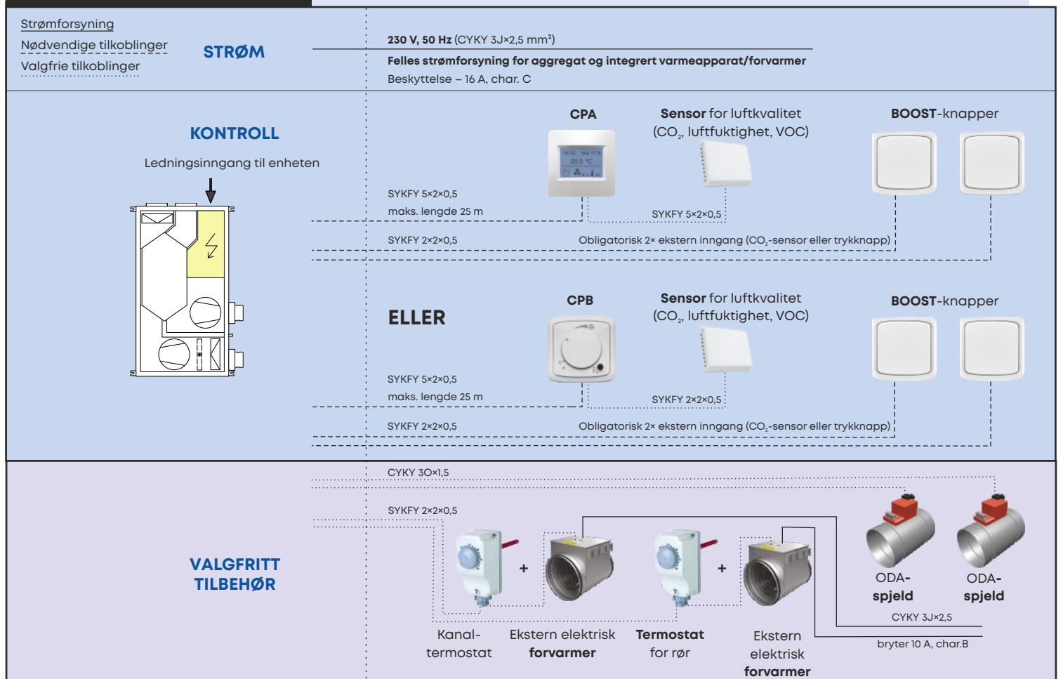
CPA regulator
