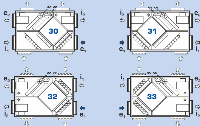
configuration 30 to 33 – top view
