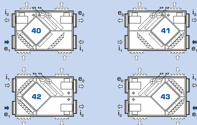
configuration 40 to 43 – top view
